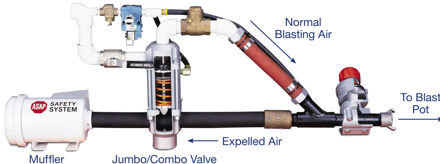
A typical ASAP System setup.
