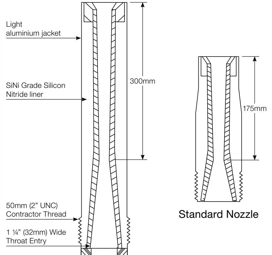
HYPER Nozzle
